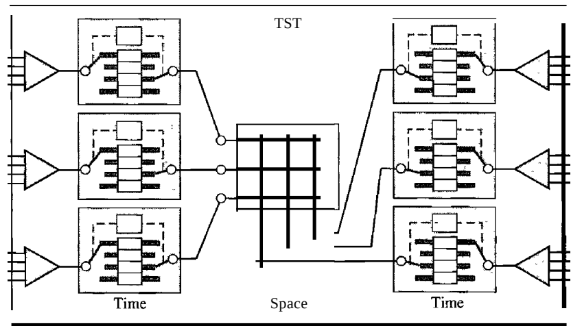
Figure 8.20 Time-space-time switch
