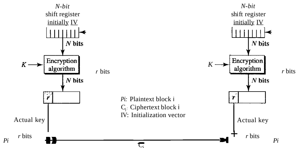
Figure 30.23 OFB mode
